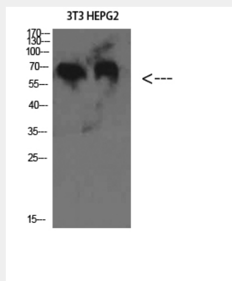
Western Blot (WB) analysis of 3T3 HepG2 cells using C8 beta Polyclonal Antibody diluted at 1:2000.
