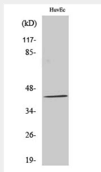
Western Blot (WB) analysis of specific cells using GALK1 Polyclonal Antibody.
