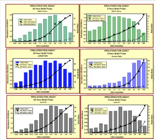
BrdU Cell Proliferation Assay Kit, detection of variable numbers of Jurkat (non-adherent) or MCF7 or RH7777 (adherent) cells per well with 2 or 24 hour pulse with BrdU. Y axis - left, OD 450-550 nm. Y axisright, signal -to-noise ratio.
