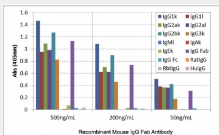
ELISA of mouse immunoglobulins shows the recombinant Mouse IgG Fab antibody reacts to the Fab region of mouse IgG1, IgG2a, IgG2b, and IgG3; no cross reactivity with IgM, IgA, IgE, human/rat/rabbit IgG.
