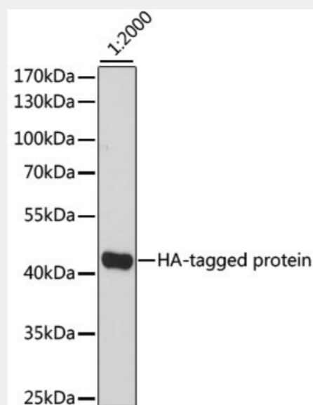
Western blot analysis of recombinant HA protein with HRP-conjugated Mouse anti HA-Tag mAb at dilution of 1:2000. Lysates/proteins: 25ug per lane. Blocking buffer: 3% nonfat dry milk in TBST.
