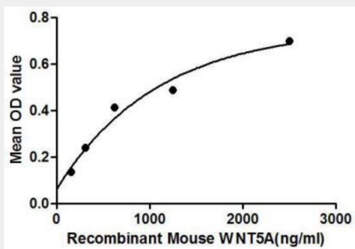
Figure 1. The binding activity of WNT5A with WIF1.
