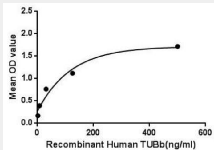
Figure 1. The binding activity of TUBb with MX1.
