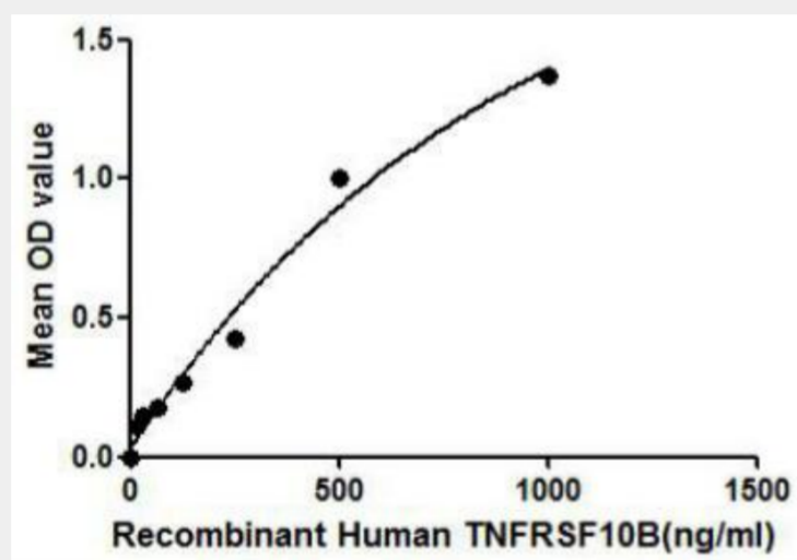
Figure 1. The binding activity of TNFRSF10B with TNF \alpha
