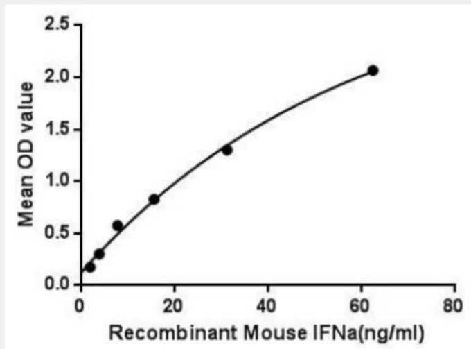
Figure 1. The binding activity of IFNa with IFNA13.
