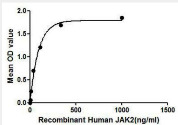
Figure 1. The binding activity of JAK2 with EPOR.
