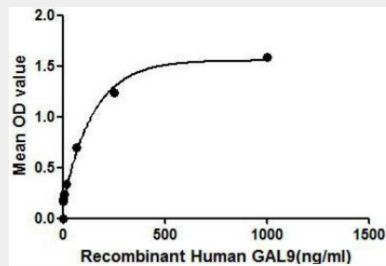
Figure 2. The binding activity of GAL9 with PDI
