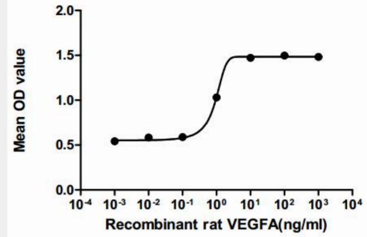
Figure 2. The dose-effect curve of VEGFA on ECV304 cells.
