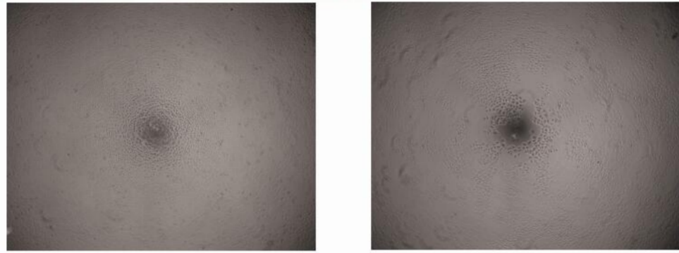
Figure 1. Cell proliferation of ECV304 cells after stimulated with VEGFA.
